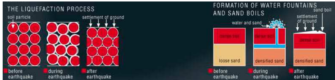
Figure 4: A representation of the liquefaction process (source: Environment Canterbury)
